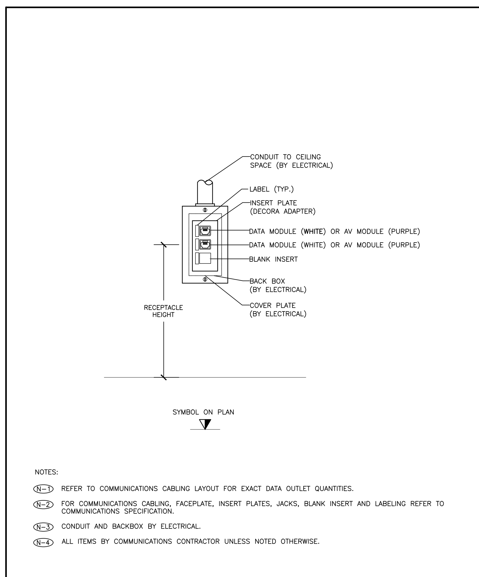
16 TYPICAL WALL MOUNTED COMMUNICATIONS 3-PORT OUTLET DETAIL TC-0.1 SCALE: N.T.S.
