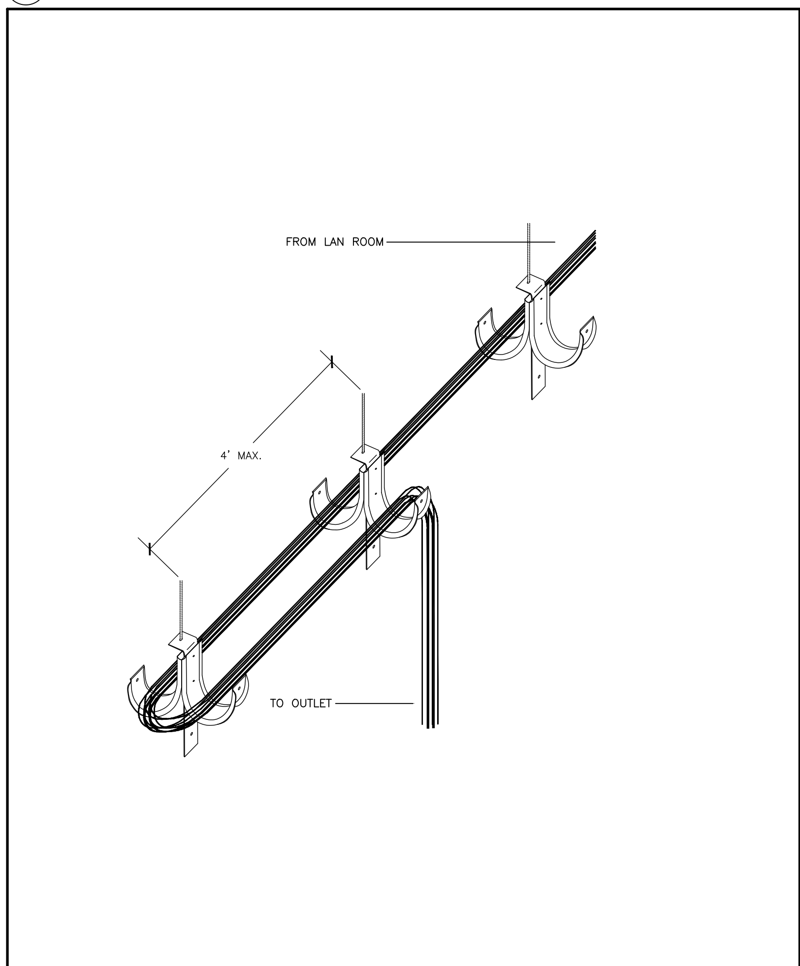
11 DUAL J-HOOK WITH PROPER COILED SLACK TC-0.1 SCALE: N.T.S.
