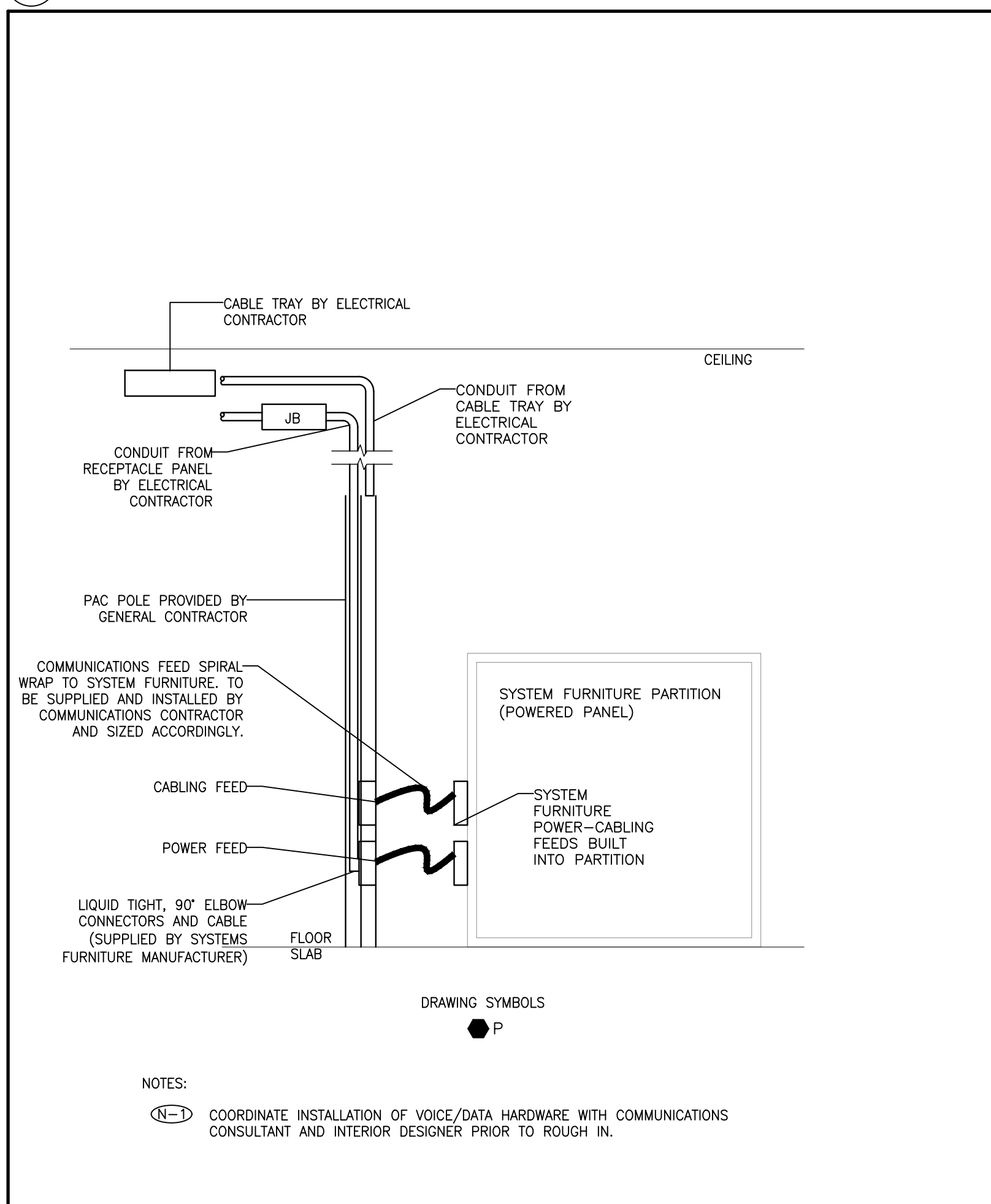
14 PAC POLE SYSTEM FURNITURE FEED TC-0.1 SCALE: N.T.S.
