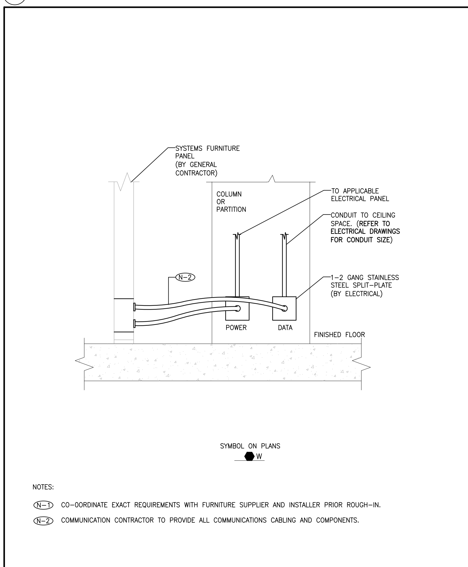
15 FURNITURE SYSTEM CONNECTION - WALL FEED TC-0.1 SCALE: N.T.S.
