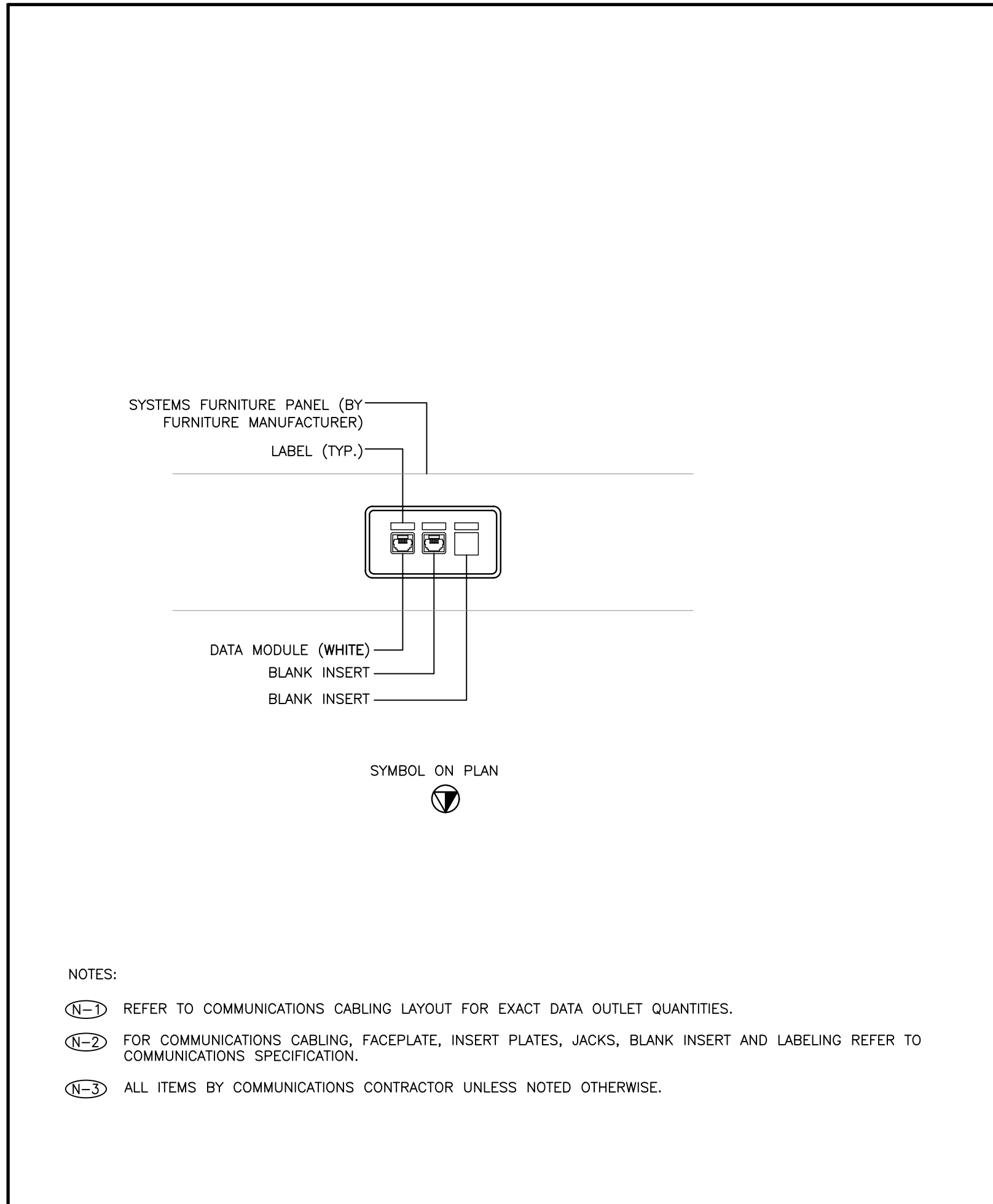
13 TYPICAL FURNITURE MOUNTED COMMUNICATIONS OUTLET DETAIL TC-0.1 SCALE: N.T.S.
