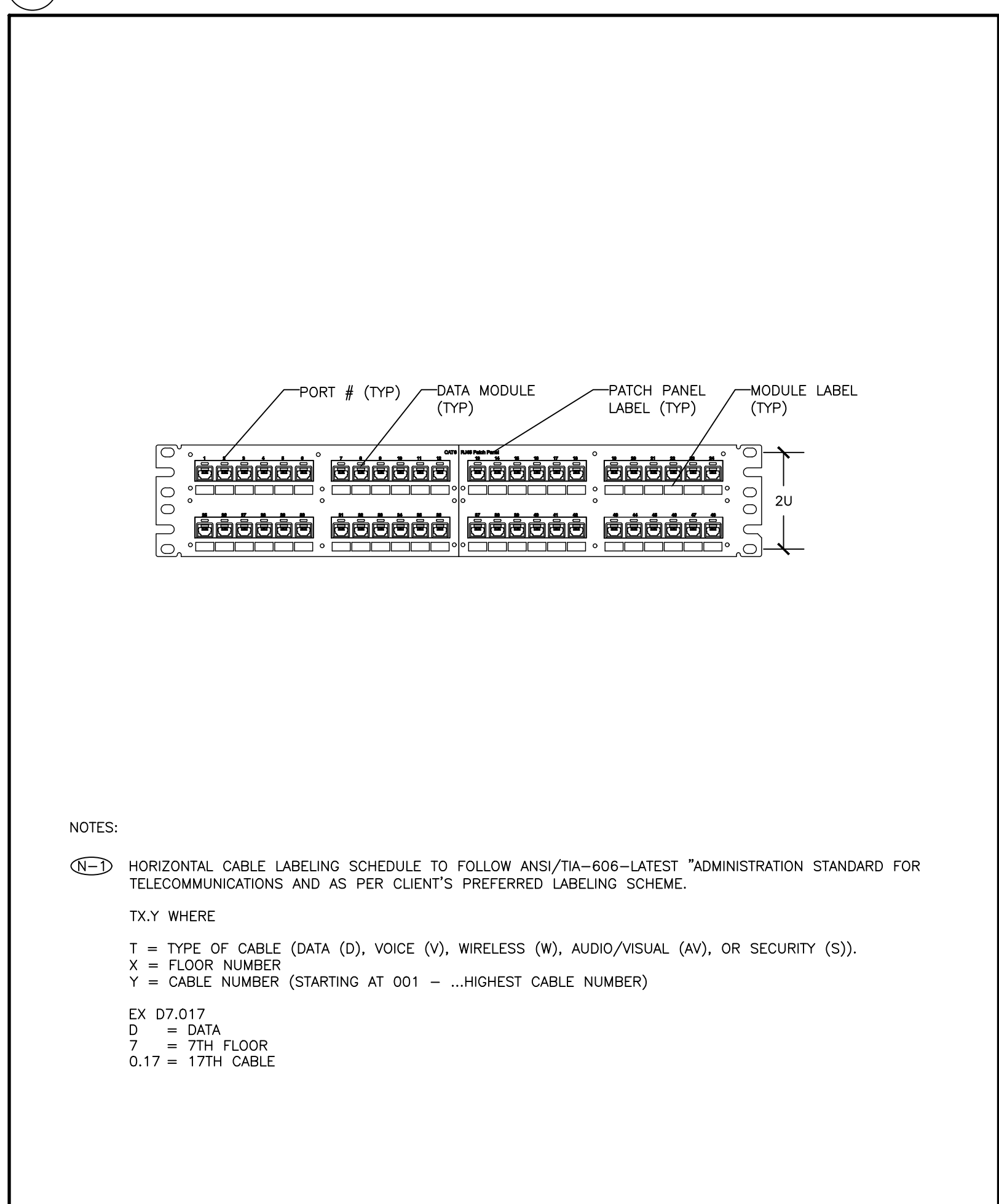
12 TYPICAL 2U-48 PORT ANGLED MODULAR PATCH PANEL DETAIL TC-0.1 SCALE: N.T.S.
