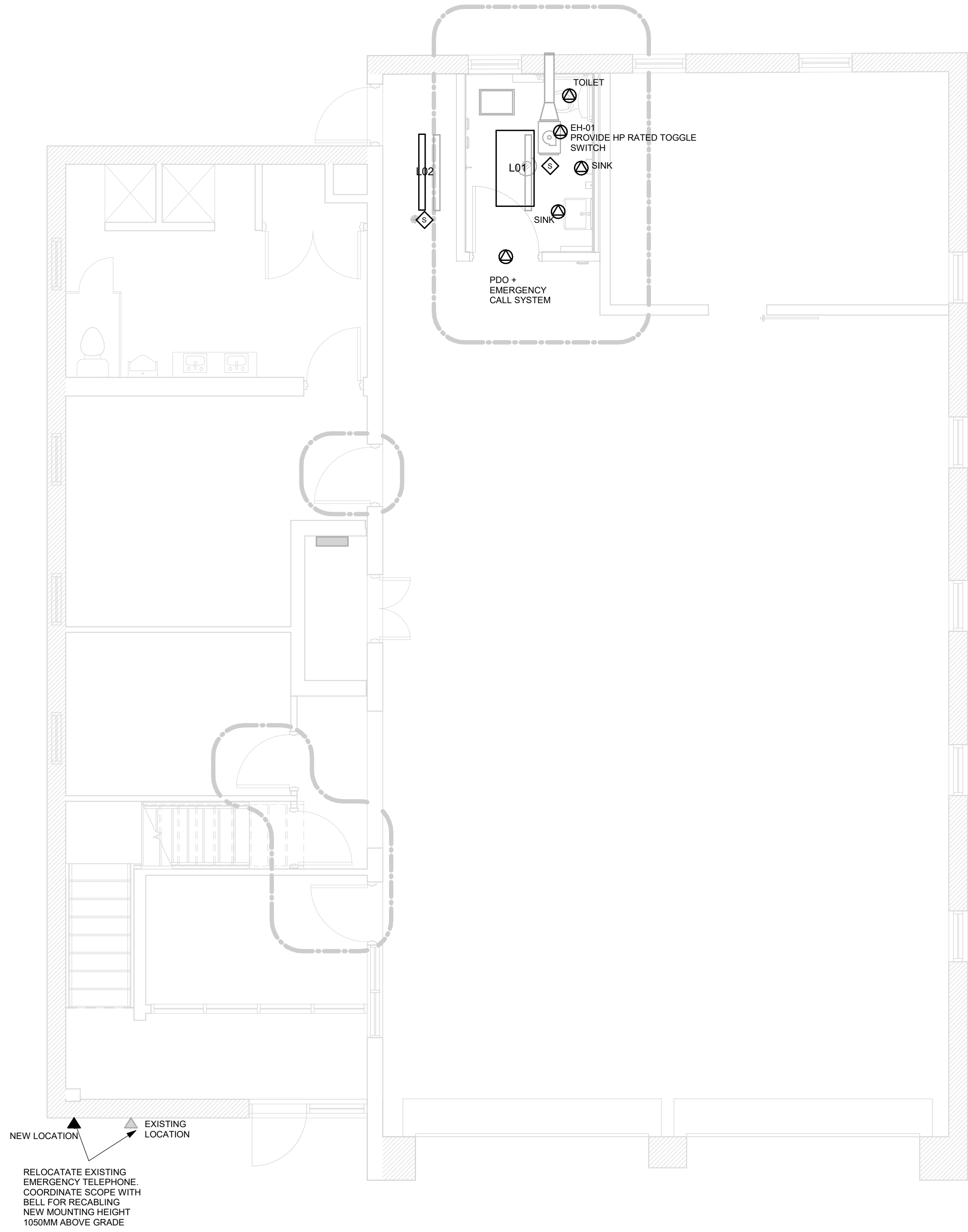
1 FIRST FLOOR POWER & SYSTEMS PLAN E2102 Scale: 1 : 50
