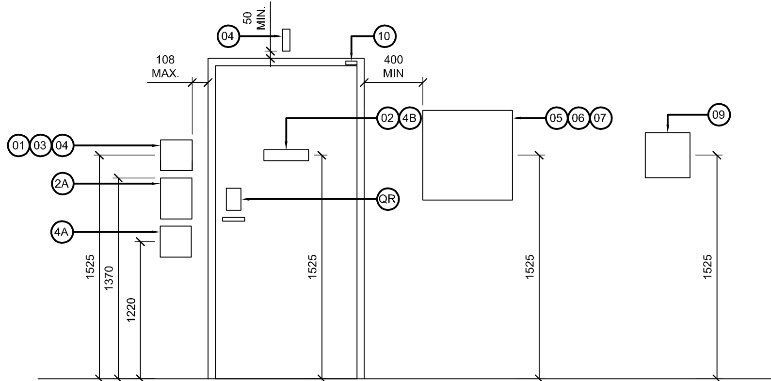
2 TYPICAL SIGNAGE ELEVATIONS ID12 SCALE: 1:25
